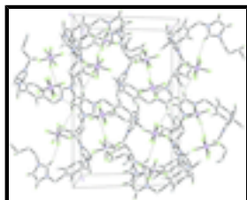
Fig. 2. The crystal packing of the title compound, showing a hydrogen-bonded (dashed lines) network. Only atoms of the major disorder components are shown for clarity.
